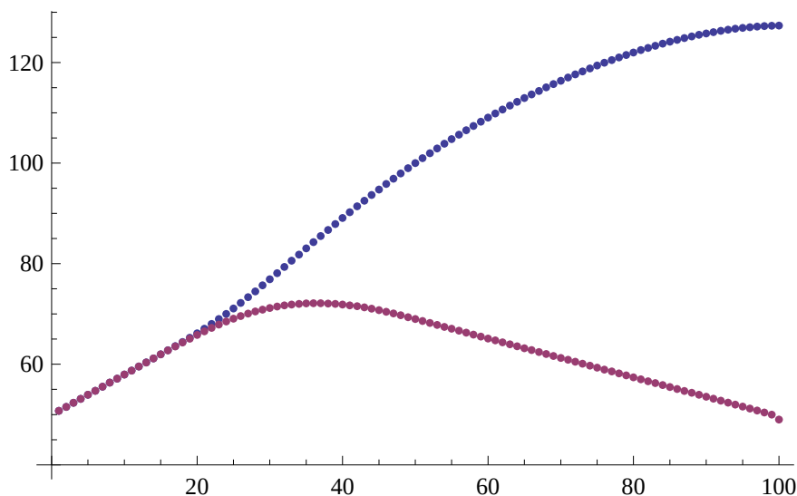
The two largest eigenvalues of M(50, k) for k = 1, 2, \dots, 100 .
